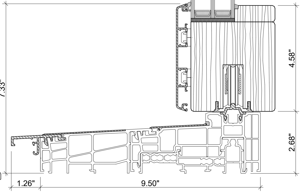
LIFT/SLIDE DOOR
