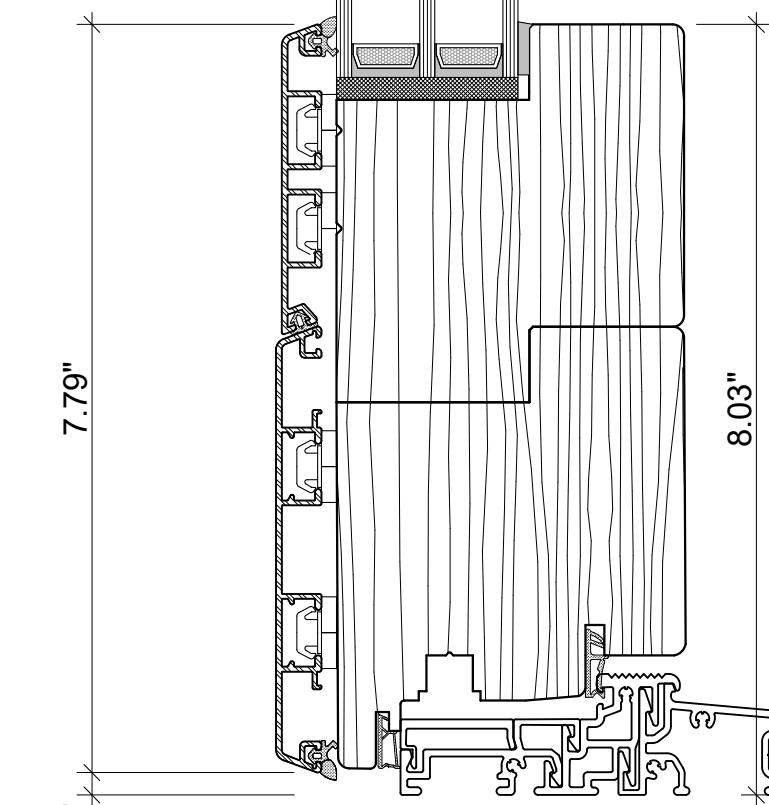
OUTSWING DOOR
