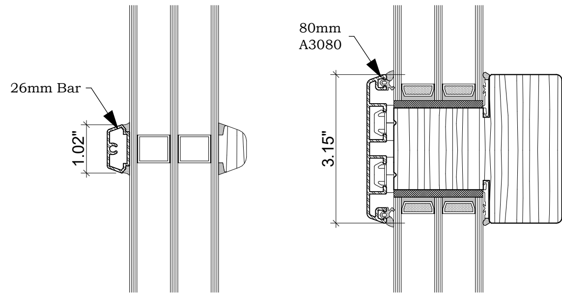
GLAZING BAR & FIXED MULLION
